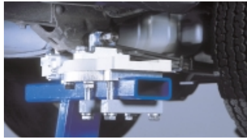
B260 clamp holds tightly to the spring shackle without removing the spring. Saves time and expense.
