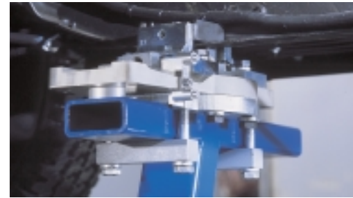
Vice-like clamp holds all frames effortlessly and precisely without collapsing the rails.
