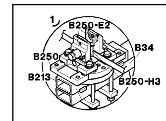
Line drawings on data sheets show exactly how and where to mount the clamps.
