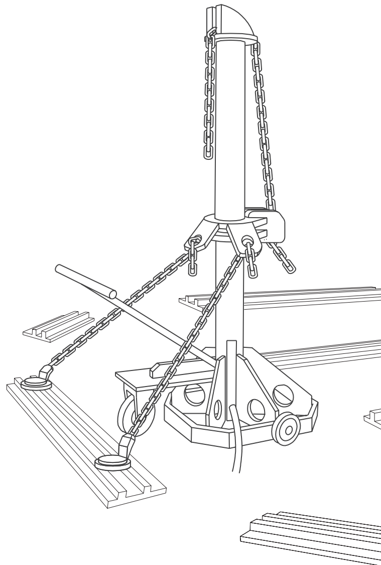
Detail of anchor pot.
